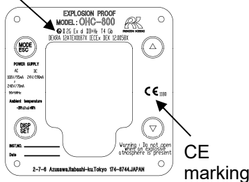
Overseas explosion-proof spec (ATEX/IECEX/China Ex, CE marking) name plate
