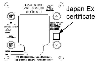
Japanese explosion-proof spec name plate
